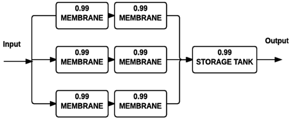
Figure 30. RBD of Membrane Elements
