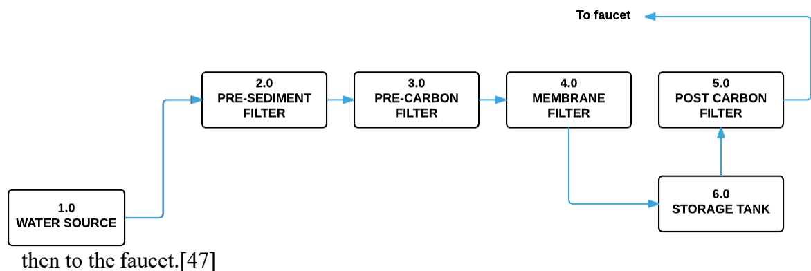
Figure 24. Block Diagram of Water Purification Mode Prototype Model
