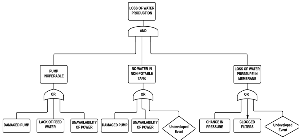
Figure 32. Fault Tree Analysis of the Water System
