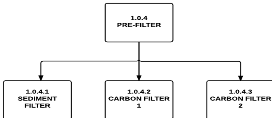
Figure 19. Physical Decomposition Level Two for the Pre-Filter Assembly
