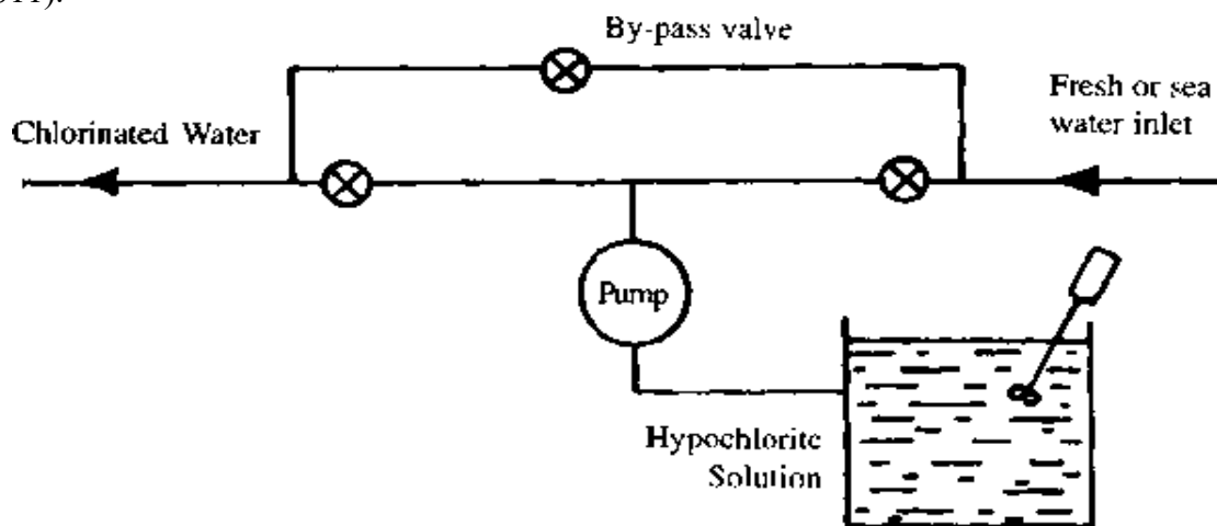
Figure 6. Chlorination Treatment. Source: Food and Agricultural Organization of the United Nations (FAO) (1999).
