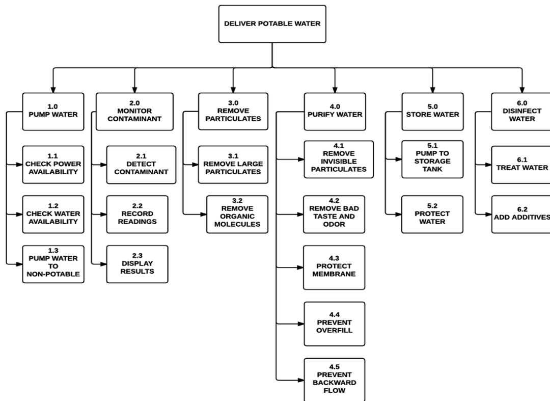
Figure 10. Functional Hierarchy of the Water System (SV-4).
