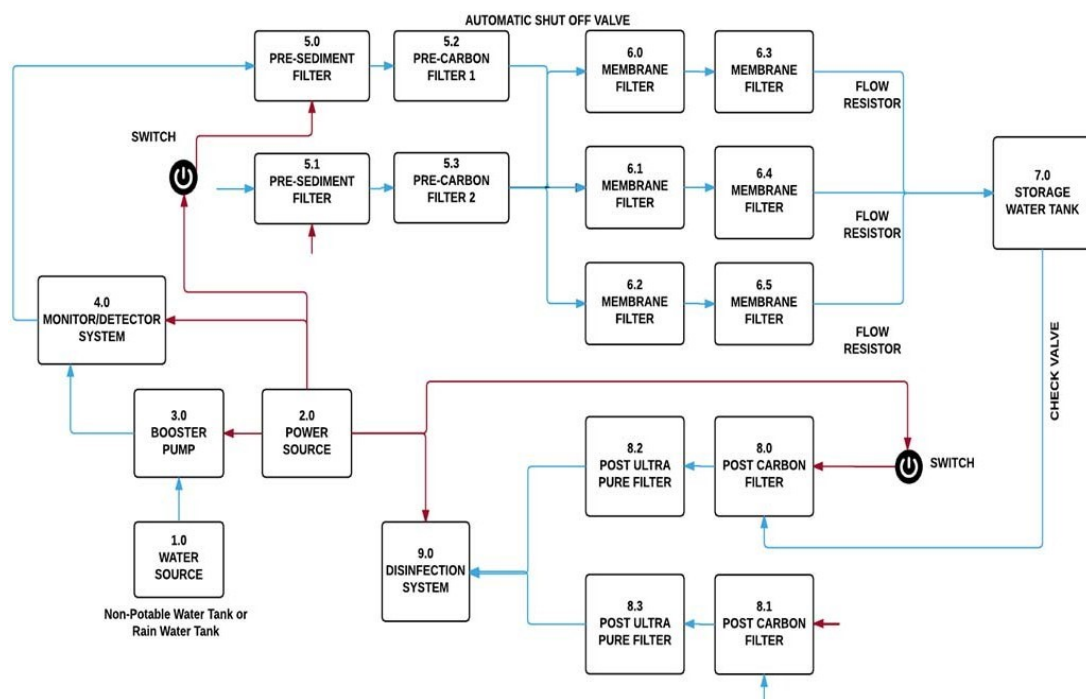
Figure 27. Water System Reliability Model
