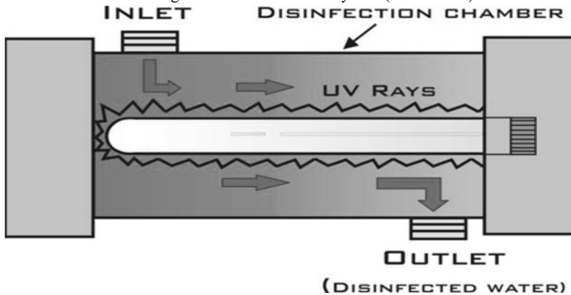
Figure 8. Schematic of the UV Water Treatment System. Source: World Intellectual Property Organization (2012).
