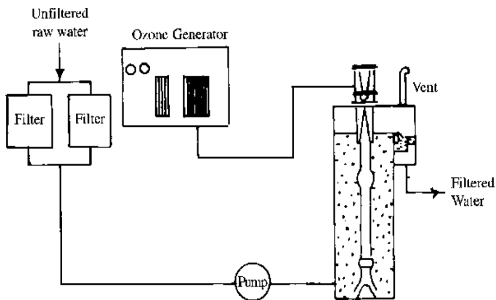
Figure 7. Ozone Water Treatment System. Source: Food and Agricultural Organization of the United Nations (1999).
