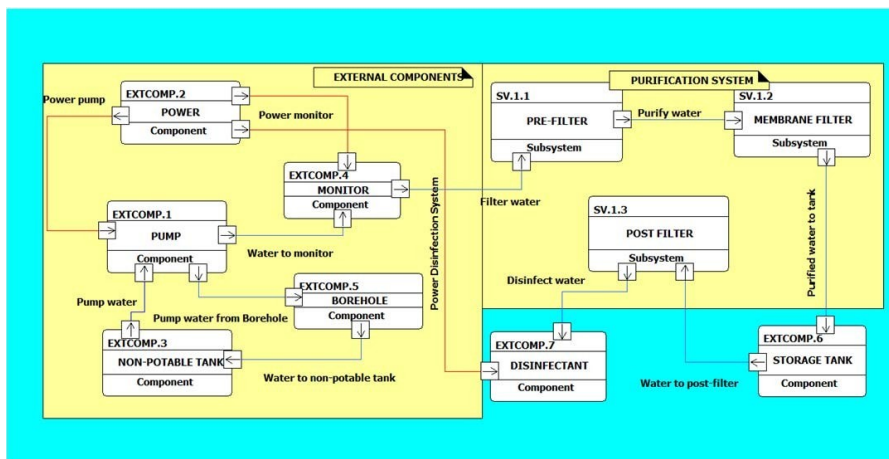
Figure 15. System Interface Diagram (SV-1)
