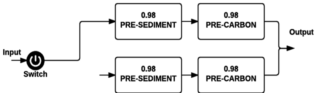
Figure 29. RBD of the Pre-filters
