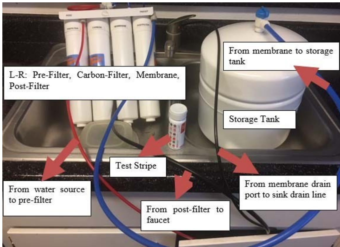
Figure 26. The Water Purification System Prototype Model Configuration
