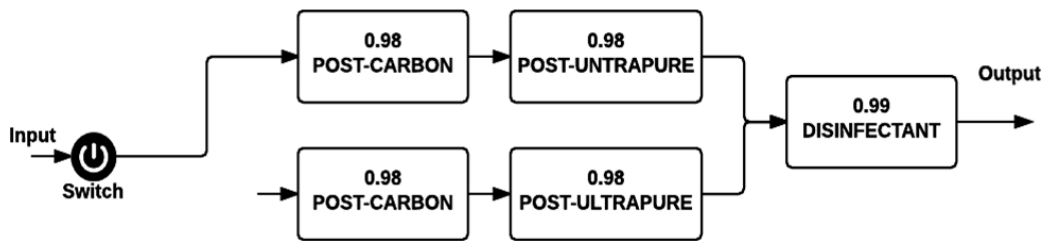
Figure 31. RBD of the Post-Filters
